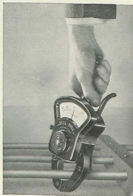
Amperímetro "Tong-Test."
